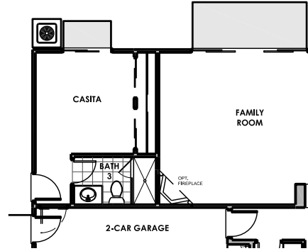
CASITA OPTION 200 SQ.FT.
