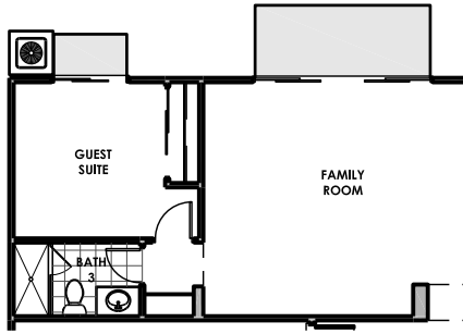
GUEST SUITE OPTION 200 SQ.FT.
